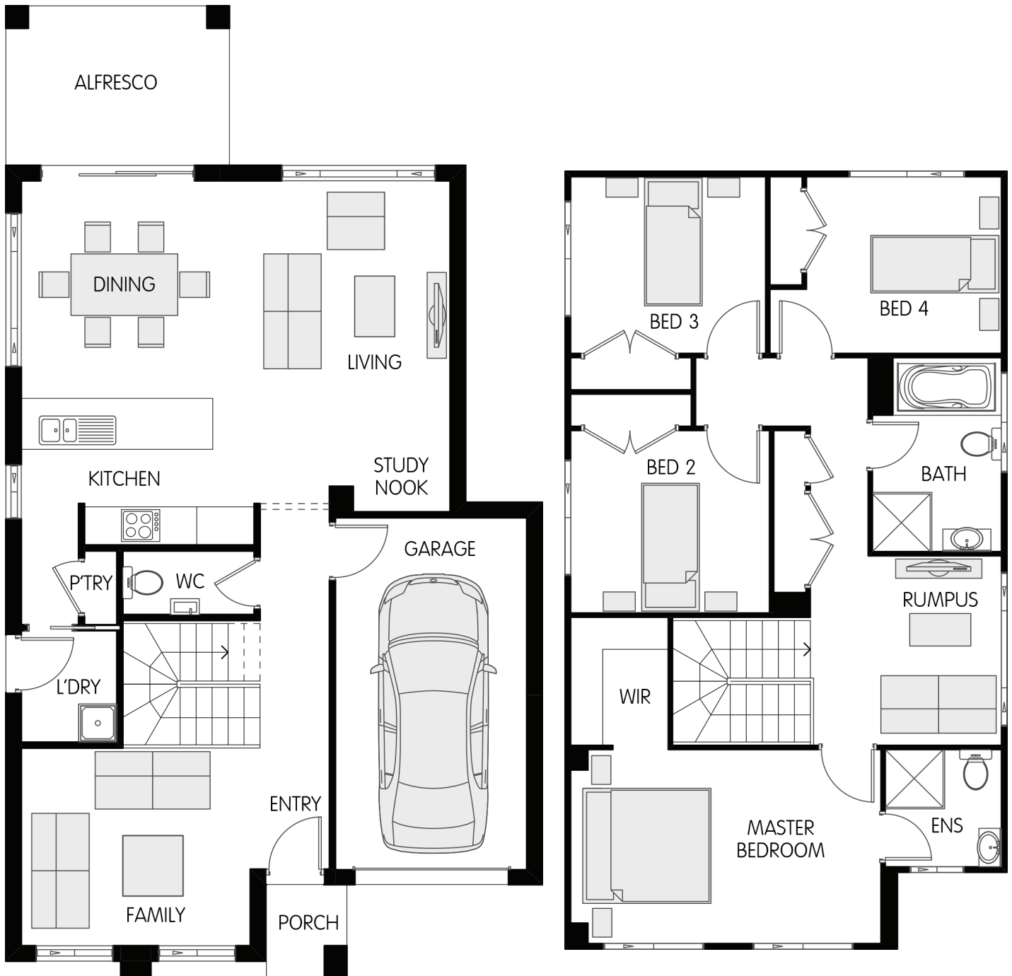
STANDARD FLOORPLAN WITH FAIRVIEW FACADE
