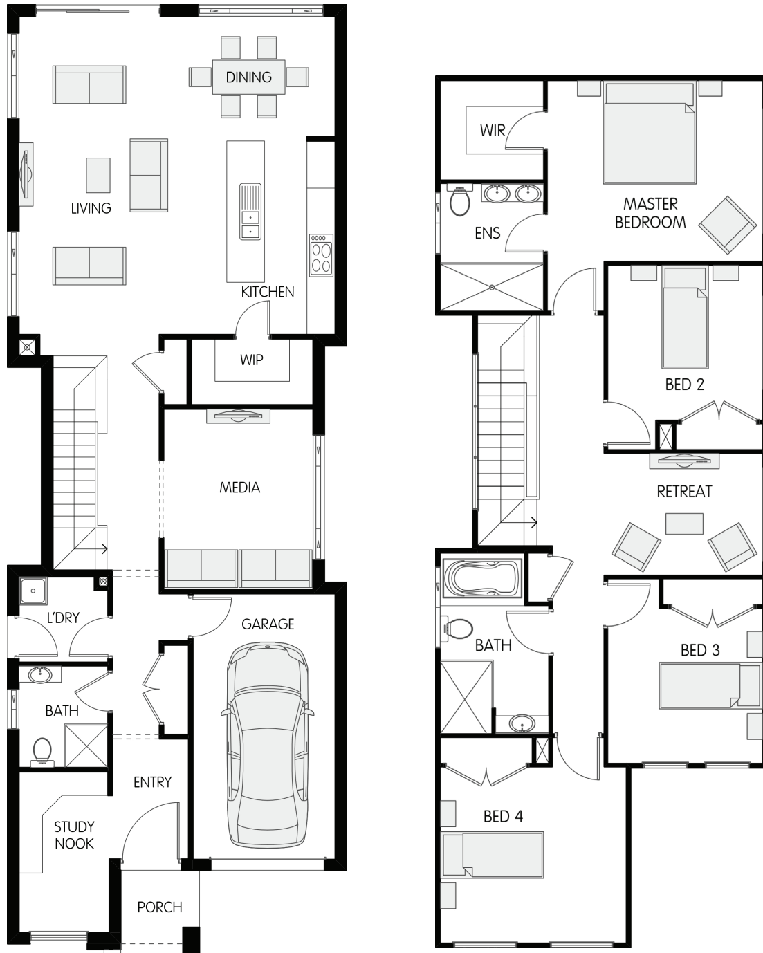
STANDARD FLOORPLAN WITH FAIRVIEW FACADE
